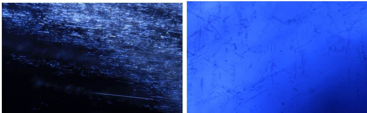
Figure 35: Detailed views of the needles and particles in GIA reference sample xx865. On the left, we see the needles in a direction perpendicular to the c-axis while on the right the needles are seen in the direction of the c-axis. Field of view 1.20mm (left), 0.94mm (right), photos: Victoria Raynaud © GIA.
