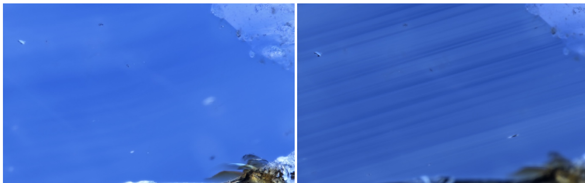
Figure 39: Left and right two different views of reference sample 100322689845 in diffused light conditions. On the left the sample looks milky but actually when it is tilted correctly bands of minute particles appear clearly. Field of view 4.32mm, photos: Victoria Raynaud ©GIA.
