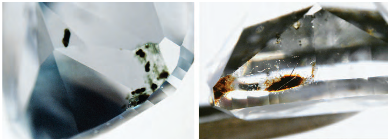
Figure 15. This 0.30 ct Fancy green-blue diamond (left) and 1.18 ct Fancy Light green-blue diamond (right), both colored by GR1 defects, show several green and brown radiation stains.
