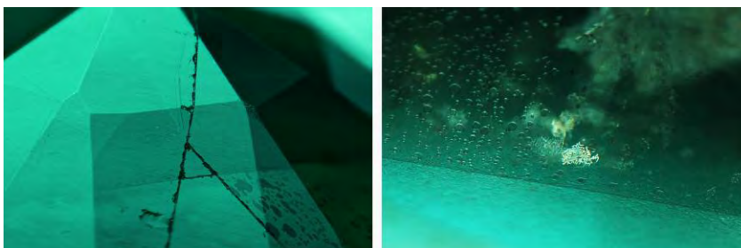
Figure 3. Left: All four glass sections of the pavilion assemblage are visible in reflected light. The small triangular segment is a protrusion from the opposite side. Field of view 3.57 mm. Right: Metallic dendritic films supporting the natural provenance of the beryl core. Also visible are planar bubbles within the cement layer. Field of view 2.90 mm.
