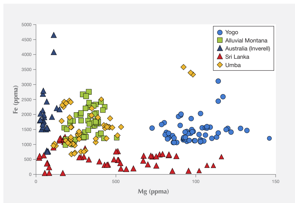
Figure 17. Plot of Mg vs. Fe (in ppma) of Yogo sapphires compared to a select group of other economically important sapphires. This generally covers the range of sapphire trace-element chemistry. Yogo sapphires have a unique chemical signature that can be used in addition to inclusions to positively identify their origin.
