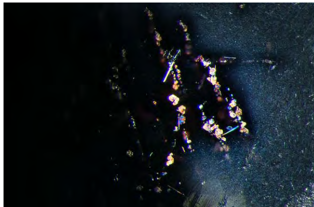
Figure 18. In the center of the image we can see larger reflective platelet inclusions in the untreated star spinel. On the right-hand side, we see much finer dense needles that form both six-rayed and four-rayed asterism. Photomicrograph by E. Billie Hughes; specimen courtesy of Global Spinel Gems.
