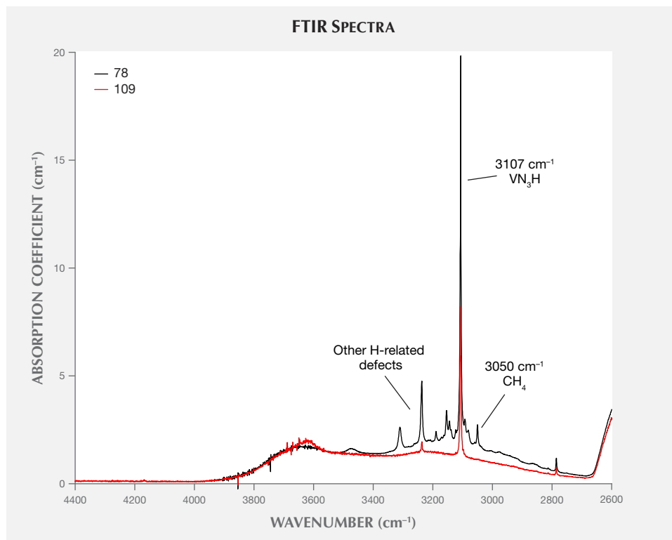
Figure 11. FTIR spectra for two representative samples that show the presence and absence of \text{CH}_4 at 3050\text{ cm}^{-1} . The sample containing \text{CH}_4 also shows other hydrogen-related peaks in the vicinity of the \text{VN}_3\text{H} peak at 3107\text{ cm}^{-1} (Goss et al., 2014). Previous work on other Marange diamonds showed that \text{CH}_4 inclusions are restricted to cuboid sectors and closely associated with the clouds of graphitic micro-inclusions (Smit et al., 2016).
