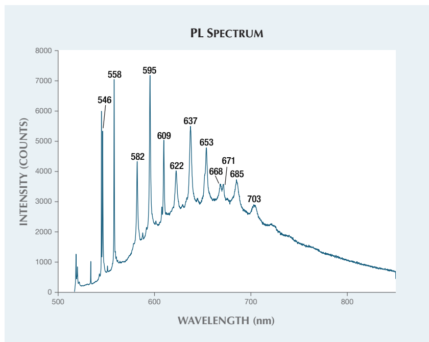
Figure 17. The PL spectrum of the 4.89 ct horse conch pearl displayed numerous peaks associated with naturally occurring polyenic pigments.
