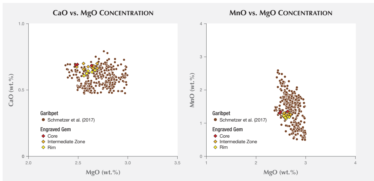
Figure 5. Binary plots showing the chemical composition of the engraved Byzantine garnet and samples from Garibpet as MgO, CaO, and MnO weight percentages.
