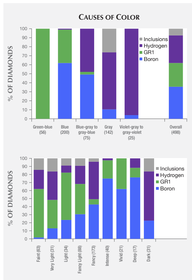
Figure 12. Natural blue/gray/violet diamonds submitted to GIA over the last decade are predominantly colored by four mechanisms. When the randomly selected subset of 500 diamonds are analyzed and divided by hue (top), clear distinctions emerge. Green-blue diamonds are comprised solely of diamonds with color due to GR1 defects, while inclusion-related defects reside only within the gray category. Diamonds with a violet component are almost exclusively due to hydrogen-related defects, and over half of the unmodified blue diamonds are type IIb. When the diamonds are segregated by tone (bottom), H- and GR1-related defects predominate within the more faintly colored diamonds while the type IIb diamonds comprise the majority of the more saturated stones. Also shown along the x-axis are the number of samples within each category.
