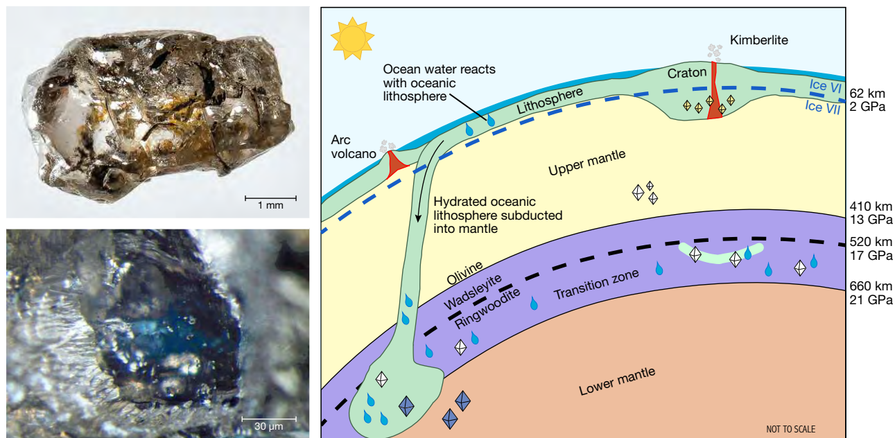
Figure 2. Ringwoodite is the high-pressure form of the mineral olivine ( \text{Mg}_2\text{SiO}_4 ) that occurs between 520 and 660 km below the surface of the earth in the transition zone. The first terrestrial observation of this mineral was in a diamond from Juína, Brazil (top left). Water content in this 30 \mu\text{m} inclusion (bottom left) is around 1.4 wt.%, indicating that the global transition zone could contain at least 2.5 times the amount of water as Earth's oceans. The majority of diamonds come from the cratonic lithosphere (indicated here as yellow diamonds). Superdeep diamonds (indicated here as white and blue diamonds) are rarer and originate from greater depths, often from the transition zone, which extends between 410 and 660 km.
