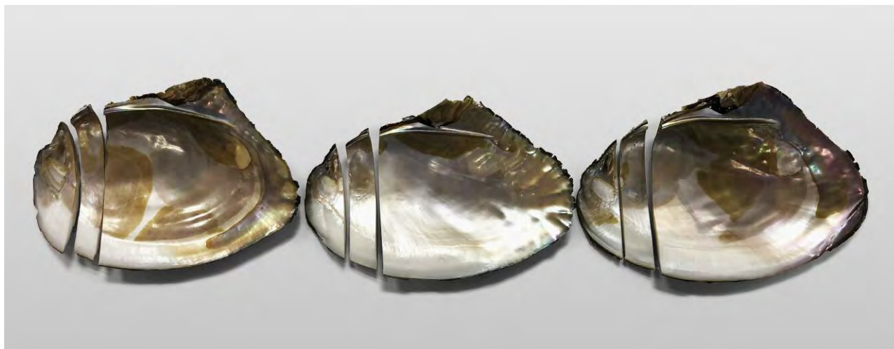
Figure 11. Three shells from Lake Kasumigaura were sliced for chemical composition analysis. The variable color and luster of the mother-of-pearl strongly influence the color of the pearl during cultivation. Photo by Ahmadjan Abduriyim.
