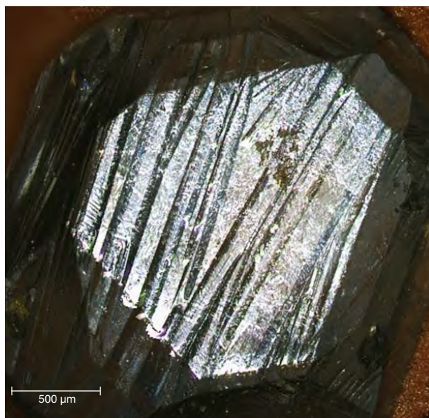
Figure 26. The surface of this HPHT synthetic diamond presents several groups of parallel lines. Photo by Xuxu Wu.
