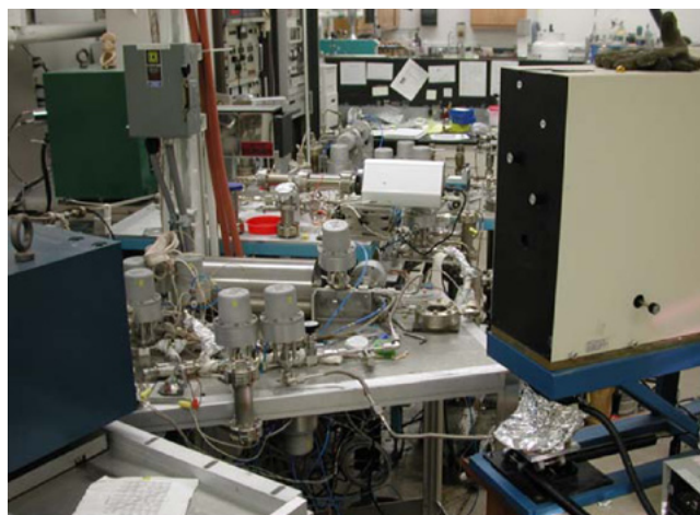
Figure 1. Laser heating system (box on the right) and gas purification system (on table) for argon analysis. Photo by George R. Rossman.
