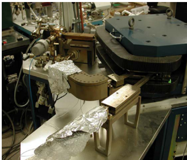
Figure 3. Mass spectrometer for Ar isotope analysis. Photo by George R. Rossman.
