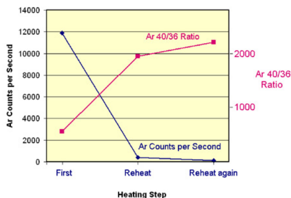
Figure 8. Reheating experiment of a red andesine rough, GRR 2635, obtained from a Bangkok gem dealer in 2008.
