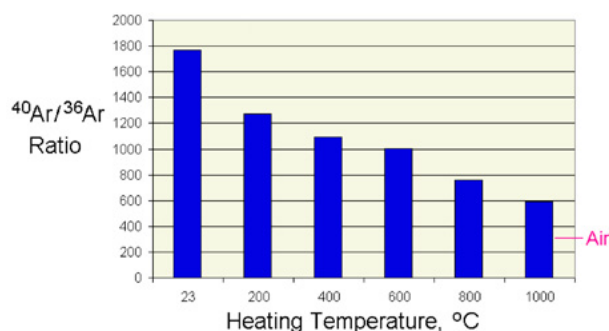
Figure 7. Argon ratios obtained from aliquots of andesine heated for 2 hours at the indicated temperature and extracted by the laser-heating method showing that some radiogenic argon remains even after heating at 1000°C.
