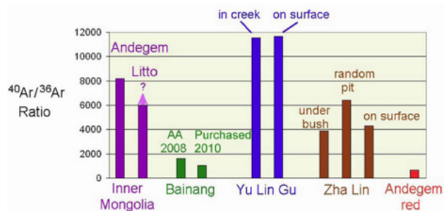
Figure 6. Results of argon extraction experiments on samples collected during the 2010 expedition, pale-yellow andesine from Inner Mongolia, a sample from the 2008 expedition to Bainang, and a faceted red gemstone.
