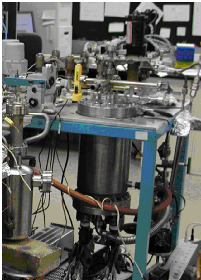
Figure 5. Furnace used to extract argon isotopes. Photo by George R. Rossman.
