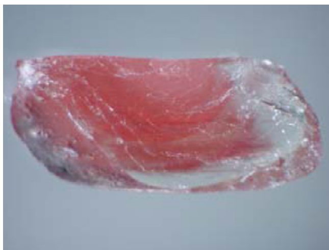
Figure 9. Andesine purchased from a villager, said to be from Bainang, Tibet. Field of view: 1.0 cm. Photo by George R. Rossman.
